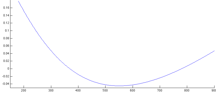
Figure 1: Relative error on the cost approximation,
