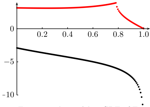
Figure 17: \lambda_+ and \lambda_- ; GRE of Fig. 3.
