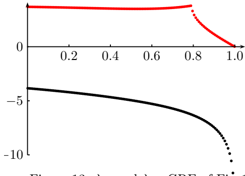
Figure 13: \lambda_+ and \lambda_- ; GRE of Fig. 1.
