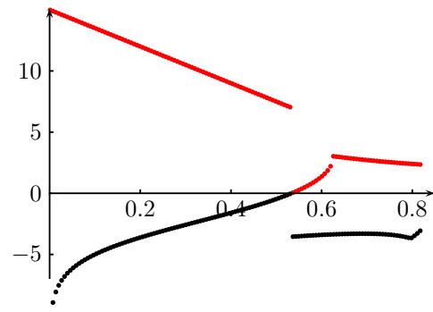
Figure 20: \lambda_+ and \lambda_- ; BGE of Fig. 4.
