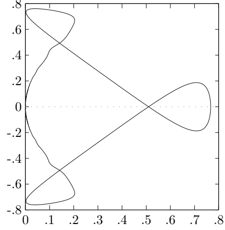
Figure 8: GRE of fig. 2, \alpha = .3
