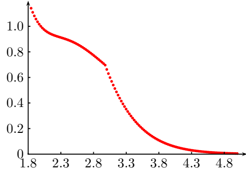
Figure 14: \lambda_+ and \lambda_- ; BGE of Fig. 1.
