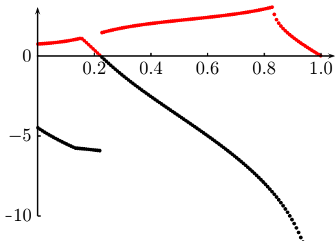
Figure 15: \lambda_+ and \lambda_- ; GRE of Fig. 2.
