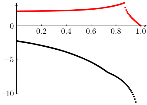
Figure 19: \lambda_+ and \lambda_- ; GRE of Fig. 4.
