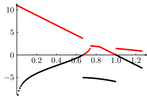
Figure 16: \lambda_+ and \lambda_- ; BGE of Fig. 2L.
