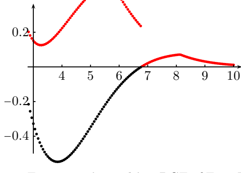
Figure 18: \lambda_+ and \lambda_- ; BGE of Fig. 2H.
