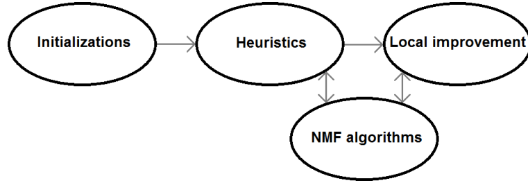
Fig. 1 Representation of the stream of the exchange of information between the different building blocks of our exact NMF heuristics. An arrow represent the transfer of a solution.
