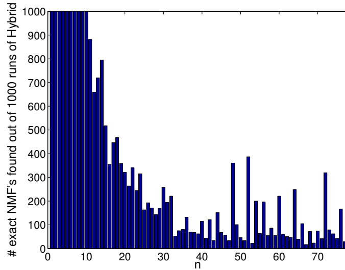
Fig. 2 Number of exact NMF found out of 1000 runs of Hybrid on regular n -gons and for the nonnegative rank given in Conjecture 2.
